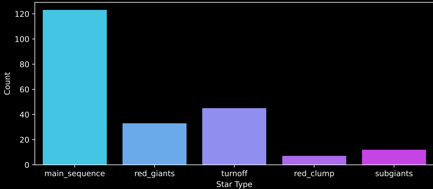
APOGEE DR17 Field: [167-55] Count plot of Star Type
