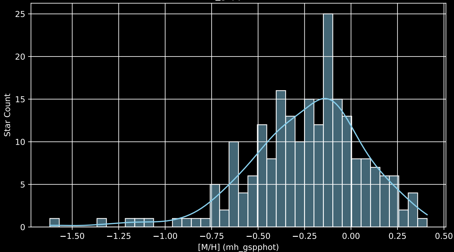
APOGEE DR17 Field: [167-55 [M/H] (mh_gspphot) (n= 217)
