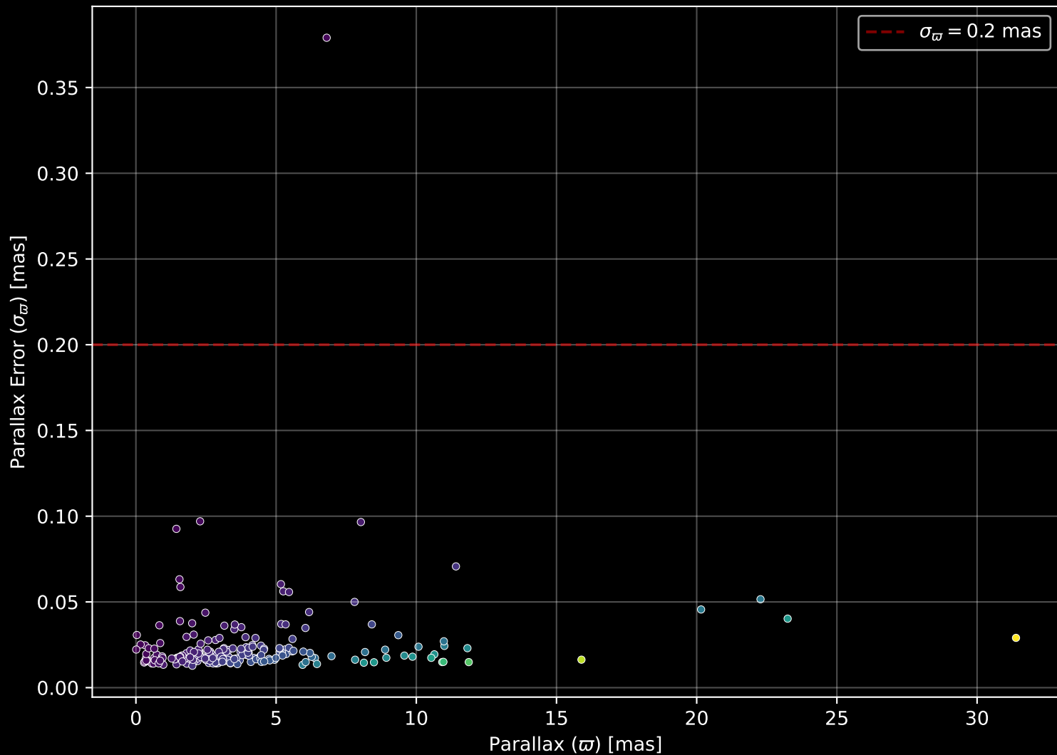
APOGEE DR17 Field: [167-55] Parallax Quality (n= 220)
