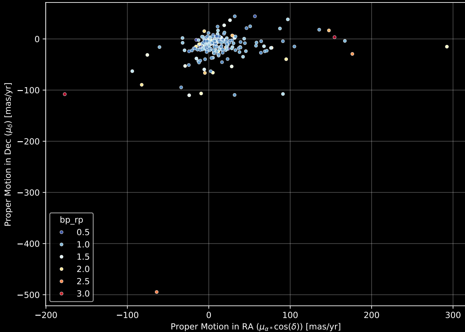
APOGEE DR17 Field: [167-55] Proper Motion Diagram (n= 220)
