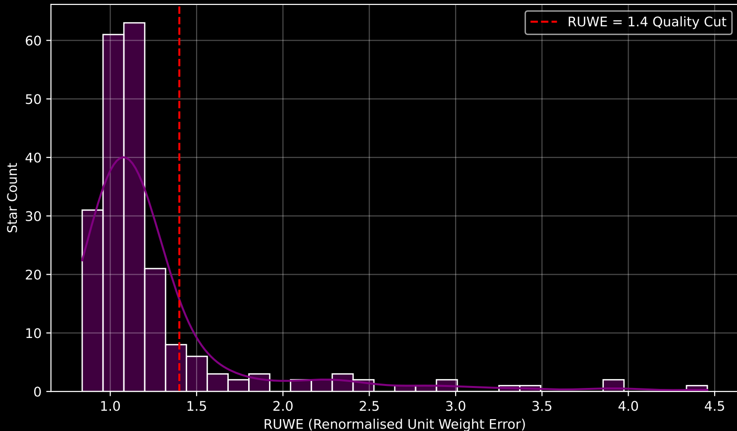
GAPOGEE DR17 Field [167-55] RUWE Distribution (n= 216)
