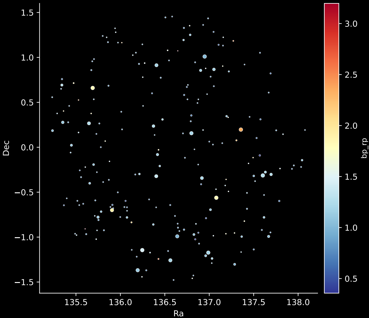
APOGEE DR17 Field: [167-55] Stars: 220
